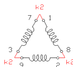
DELTA CONNECTION
