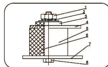
接头式B Connector Type B
