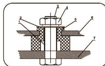
接头式A Connector Type A
