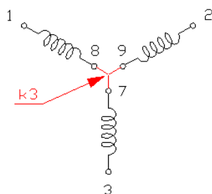
STAR CONNECTION
